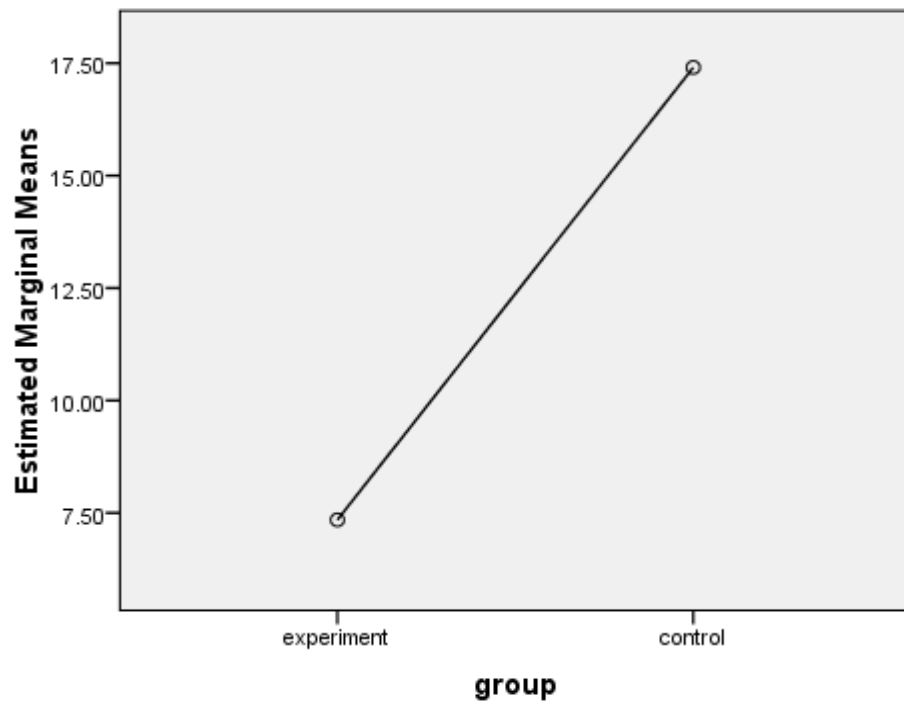
Figure 1. Difference among Estimated Marginal Means of 2 Groups
