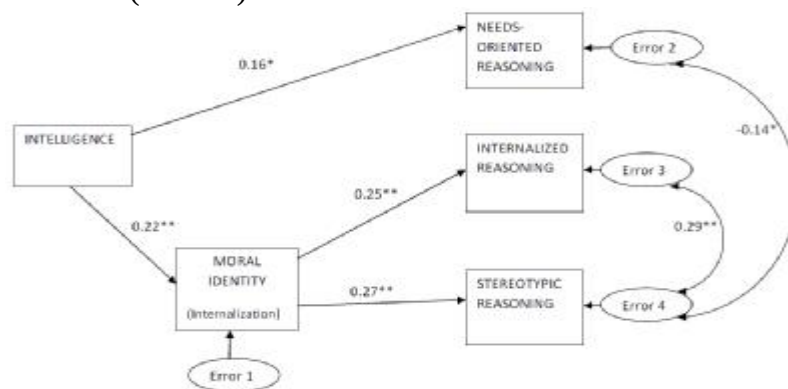
Figure 3. Standard Regression Coefficients (betas) of the Final Modified Model
